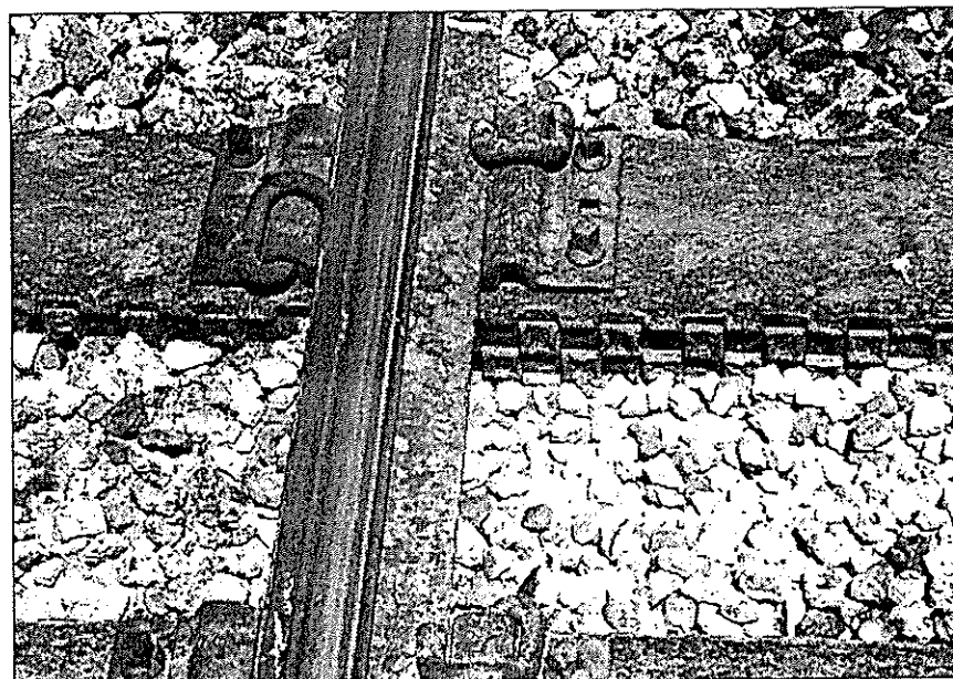
Exhibit 40. US Plastic Lumber Rough-sided Plastic Composite Tie
