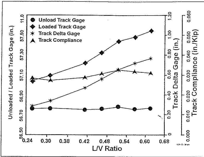
Exhibit 28. Hardwood/Softwood Ties with Four Cut Spikes, Unloaded, Loaded, Delta Gage and Track Compliance versus L/V Ratio where V=39 Kips
