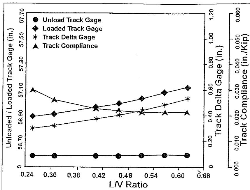
Exhibit 27. Concrete Ties with Pandrol E-clips, Unloaded, Loaded, Delta Gage and Track Compliance versus L/V Ratio where V=39 Kips
