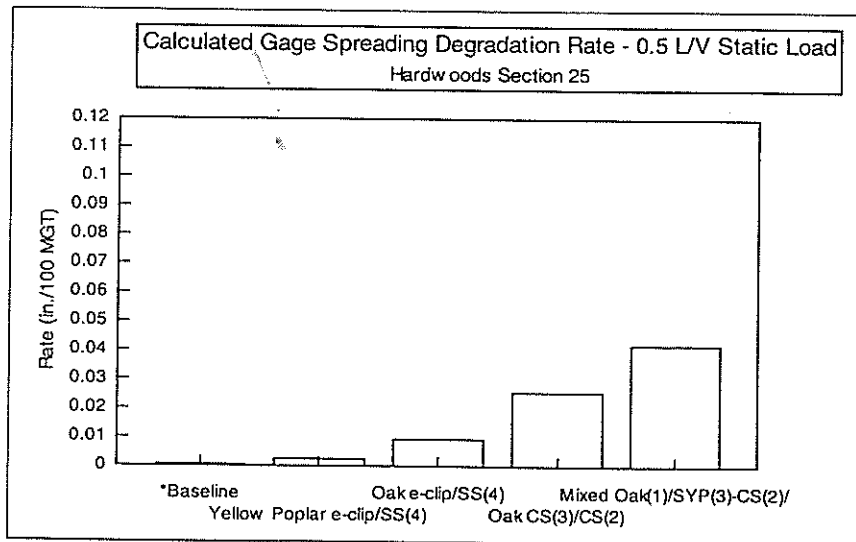
Exhibit 36. Calculated Gage Spreading Degradation Rate of Hardwood Ties under Static 0.5 L/V Load Ratio in the 6-degree Curve
