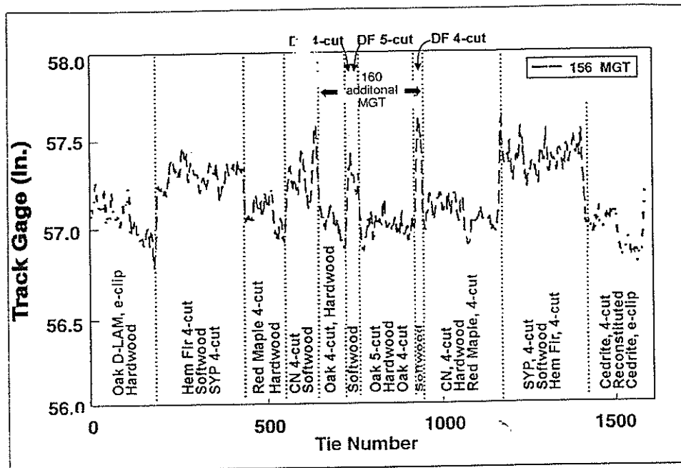
Exhibit 21. Measured Track Gage Using the EM-80 Track Geometry Vehicle
