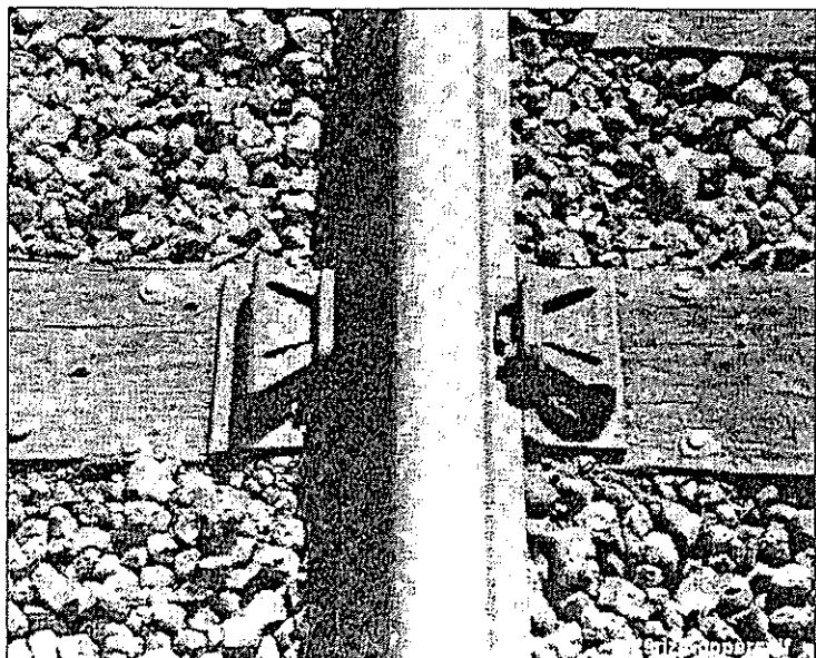
Exhibit 13. Koppers Prototype Rail Fastener
