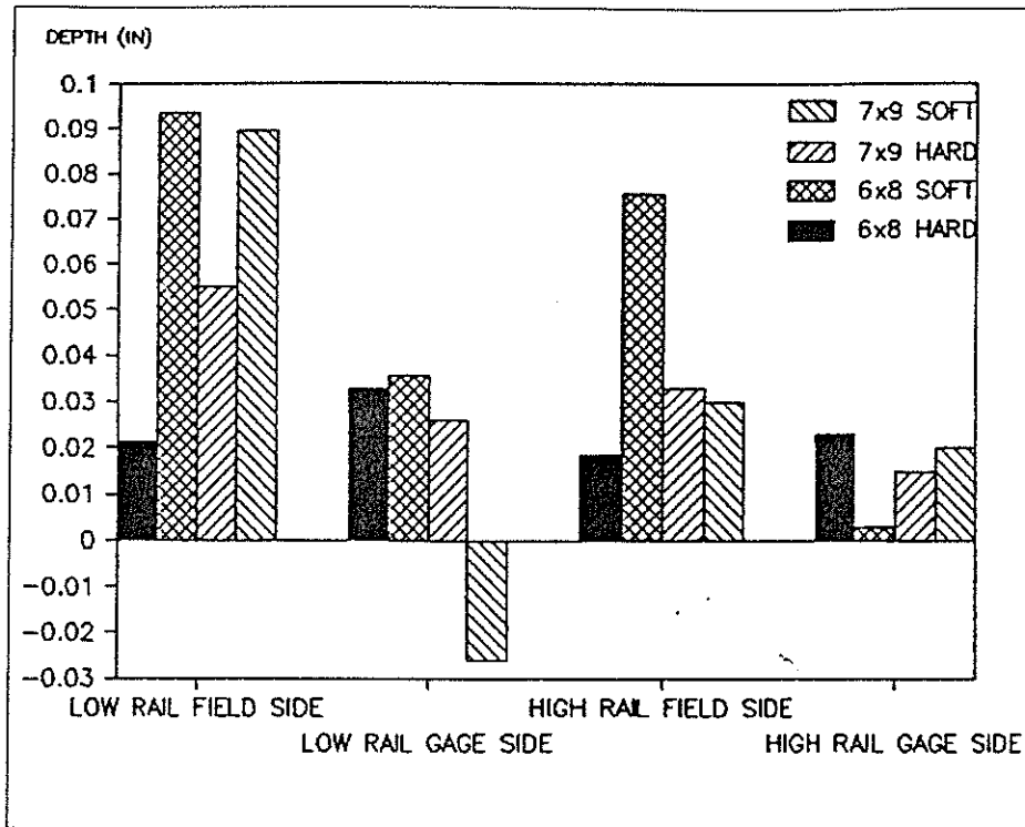
Exhibit 38. Average Tie Plate Cutting Depth on Hardwood and Softwood Ties in Section 25 after 160 MGT
