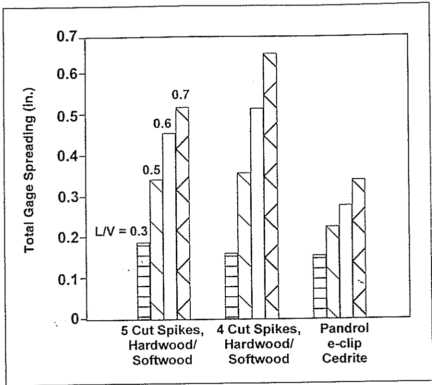
Exhibit 25. Comparison of Static Gage Spreading on Different Tie/Fastener Combinations, Section 33, Tangent Track
