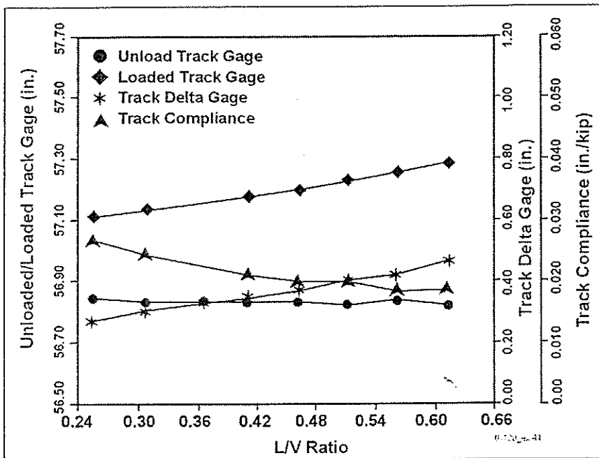
Exhibit 30. Hardwood/Softwood Ties with Pandrol E-clips. Unloaded, Loaded, Delta Gage and Track Compliance versus L/V Ratio where V=39 Kips
