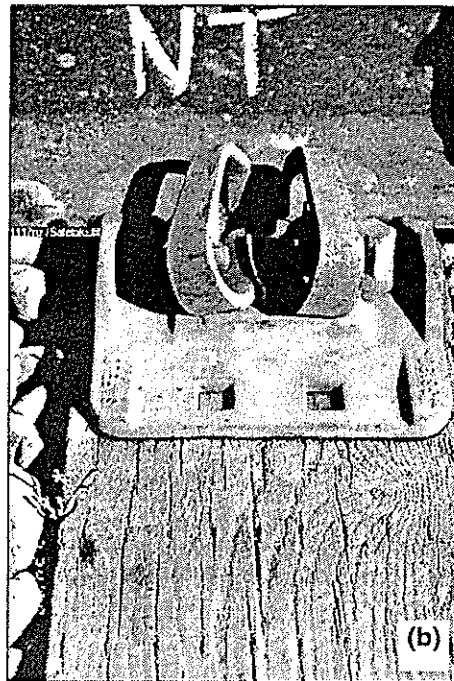
Exhibit 18. (a) One of the Rail Joints where SAFELOK® Rail Clip Fractures Occurred and (b) a Typical Fracture
