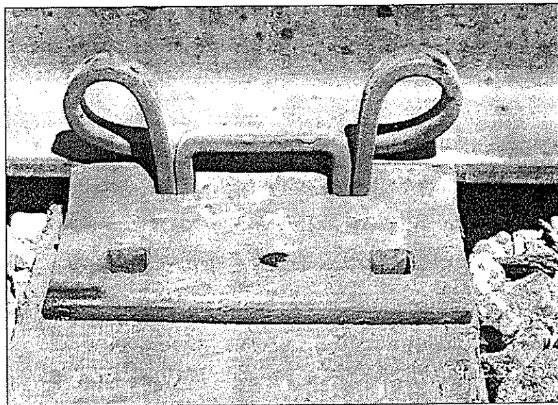
Exhibit 20. Double Elastic Fastener Similar to Those Removed from the Azobe Ties
