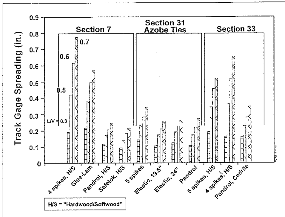
Exhibit 26. Comparison of Static Gage Spreading of Different Tie/Fastener Combinations in the Two 5-degree Curves (Sections 7 and 31) and the Section 33 Tangent Test Zone
